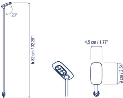
Birdie Luminaria 80S / Birdie Luminaire 80S
