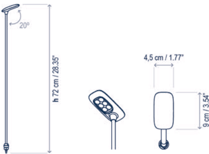
Birdie Luminaria 70S / Birdie Luminaire 70S
