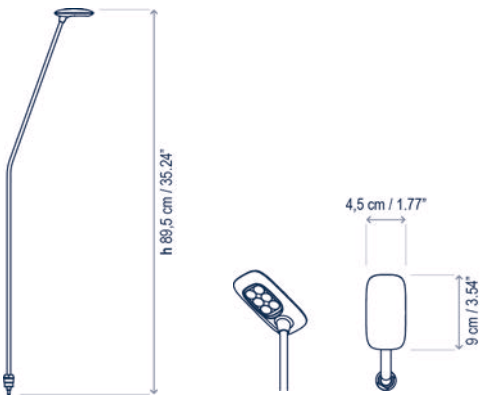
Birdie Luminaria 90SC / Birdie Luminaire 90SC
